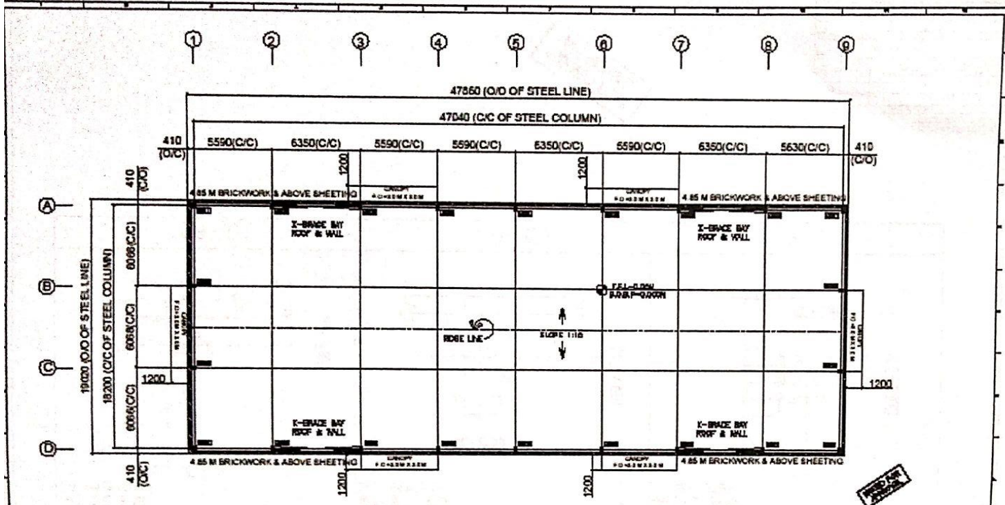
ANCHOR BOLT PLAN
